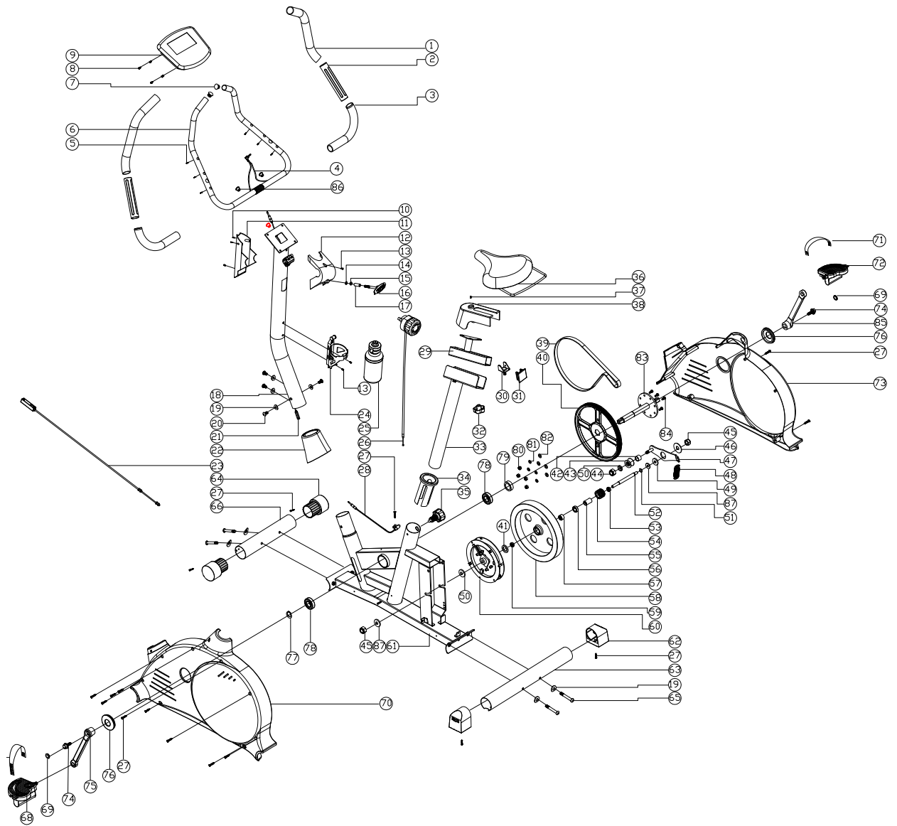
CB516-V2 exploded diagram
